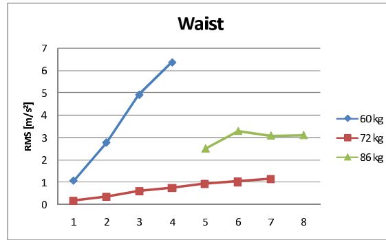
Figure 10: Vertical accelerations (RMS) for the waist zone (subject tests)
